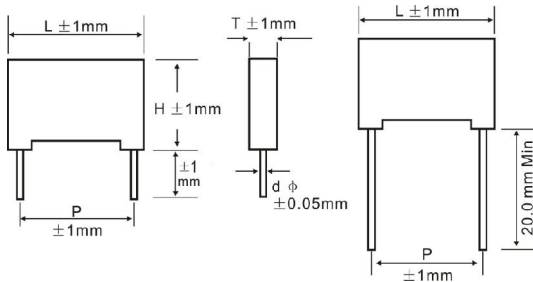
Dimensions Table for 310V AC:
